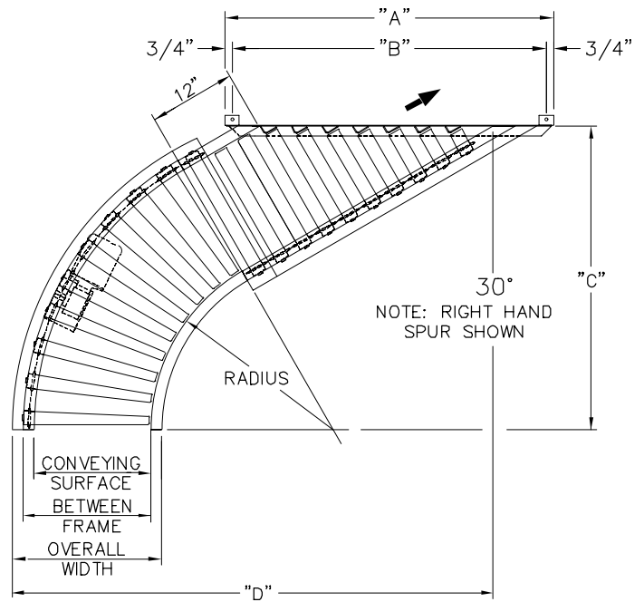
MODEL "22CRRCs" - 30° CURVE SPUR
